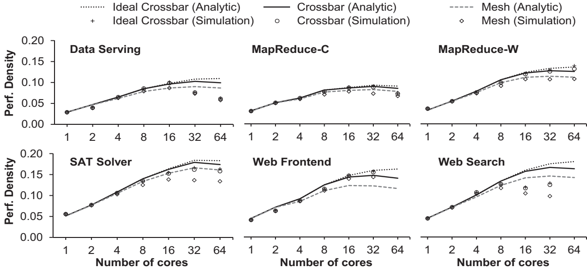
Figure 5. Cycle-accurate simulation and analytic results for designs with out-of-order cores and a 4MB LLC.
